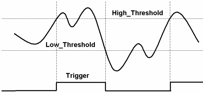
Figure 46: High-Hysteresis analog trigger condition
