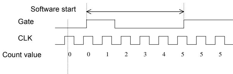
Figure 35: Mode 2 Operation
