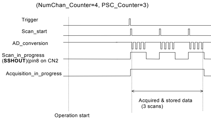
Figure 21: Post trigger
