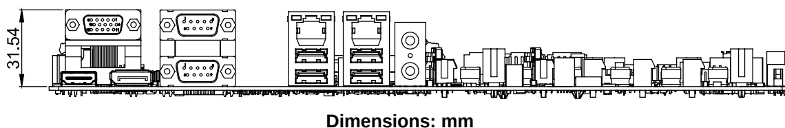
Figure 5: Mechanical Dimensions - IO Panel
