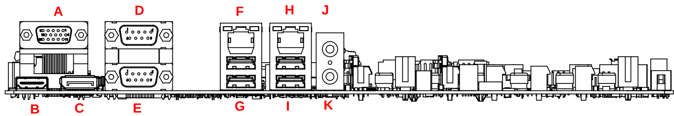
Figure 2: IO Panel Connector Locations
