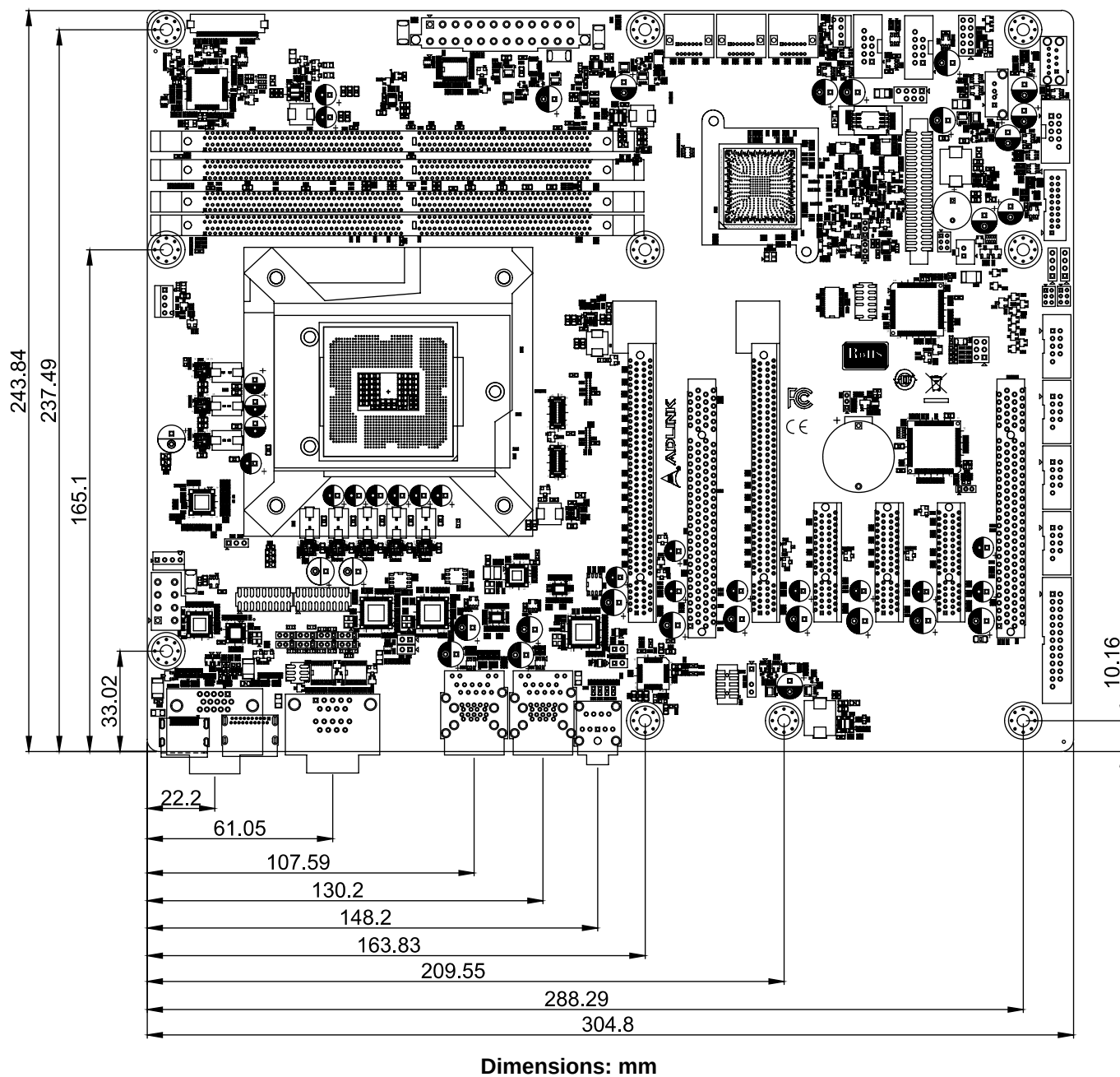
Figure 4: Mechanical Dimensions
